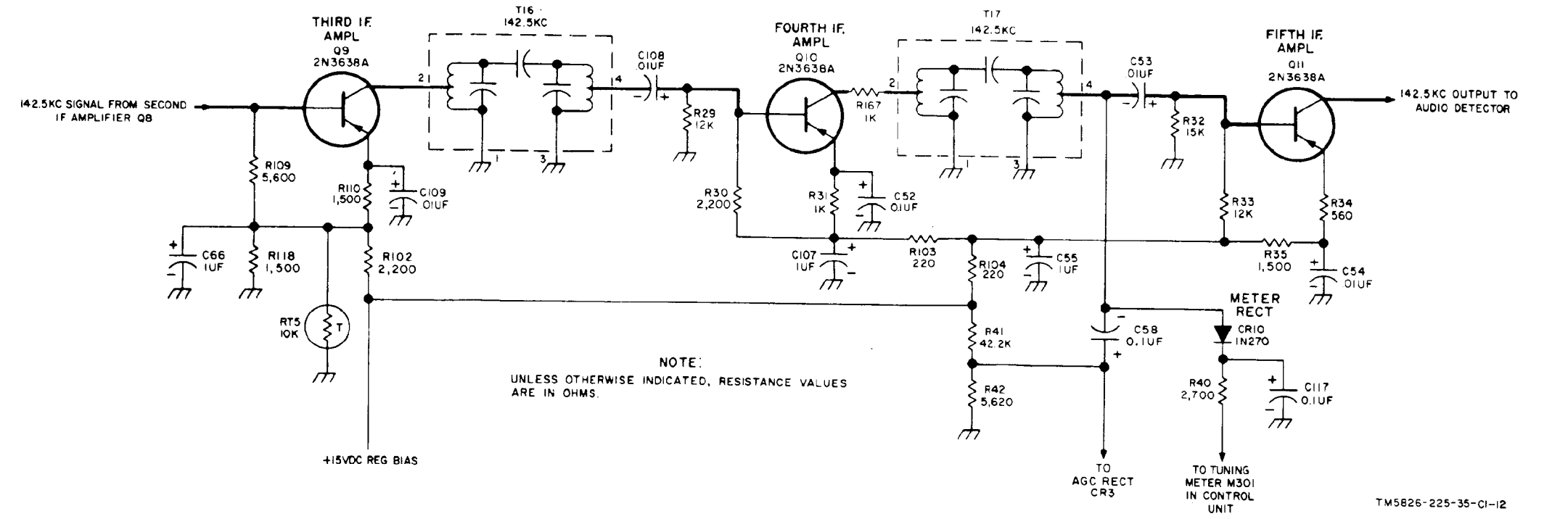
Figure 5-8. Third, fourth, and fifth IF amplifiers, schematic diagram.
