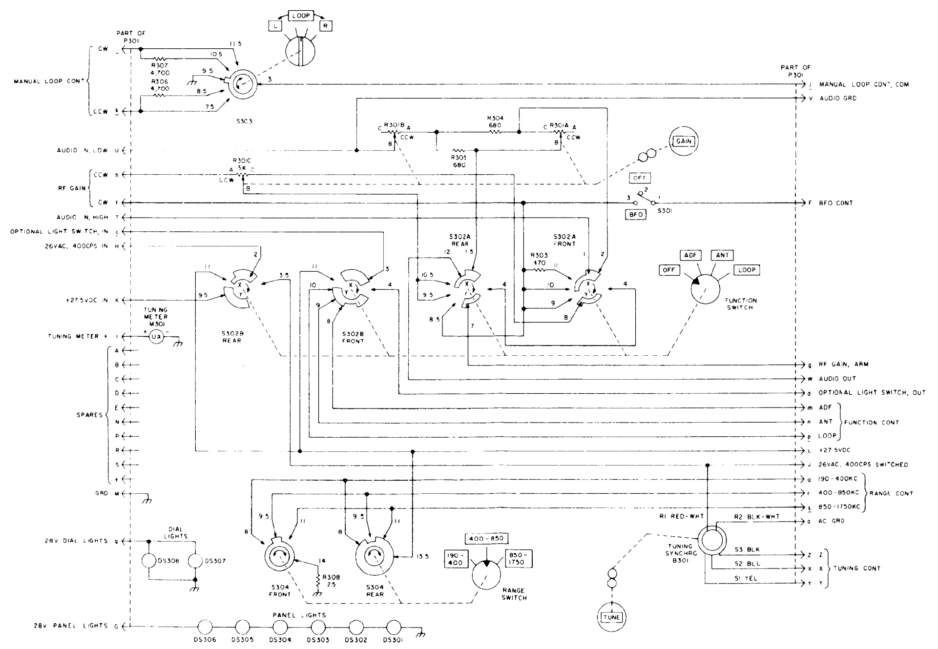
Figure 5-11. Direction Finder Control C-6899/ARN-83, schematic diagram.
