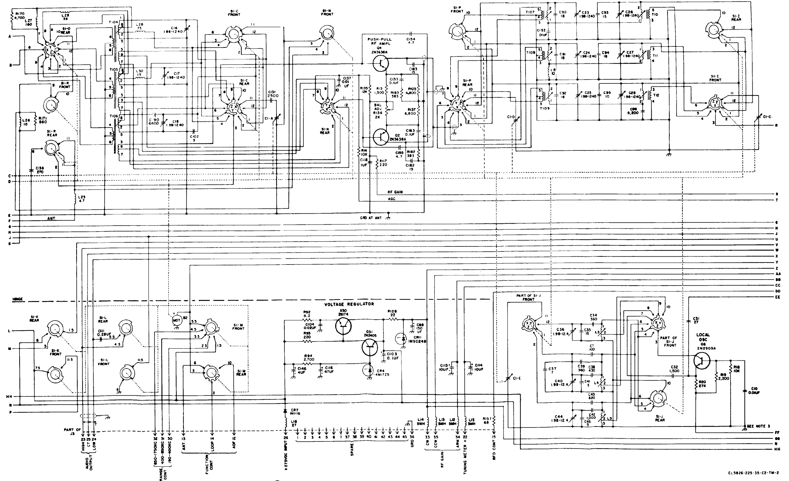
Figure 5-10.4 Radio Receiver R-1391/ARN-83 (CPN 522-2587-015), schematic diagram (sheet 2 of 3).
