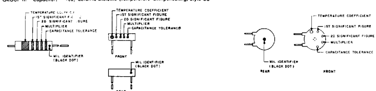
Figure 8-1. Color code marking for MIL-STD capacitors.
